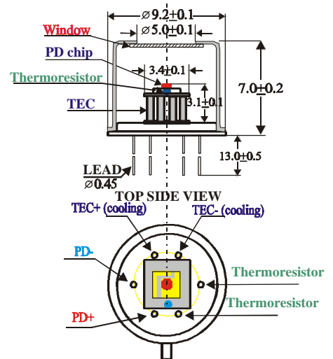
Package TO-5
