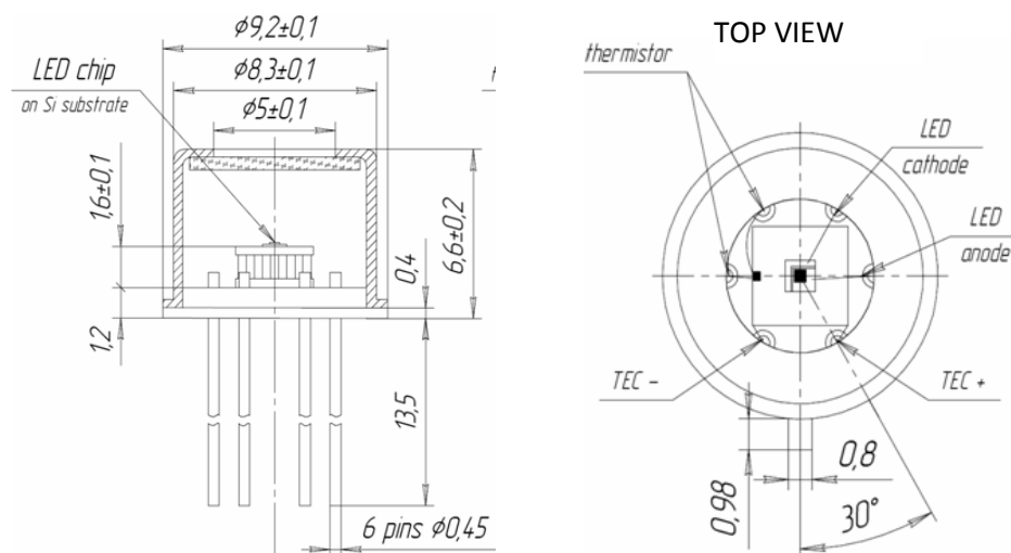
Dimension Drawing (units: mm)
