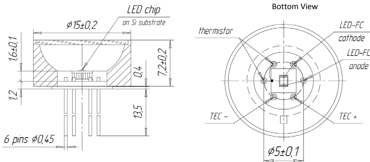
Dimension Drawing (units: mm)
